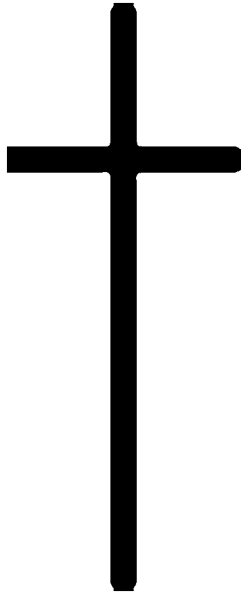
Figure 27-3 Order = O → H → L → C.
