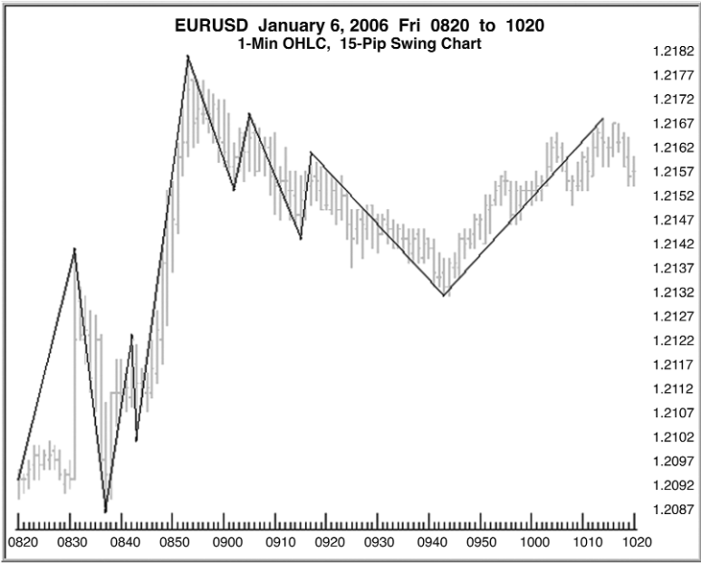
Figure 29-3 EURUSD 01/06/2006 15-Pip Reversal Amount.
