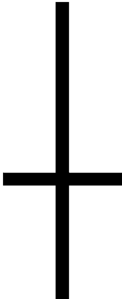
Figure 27-4 Order = O → L → H → C.
