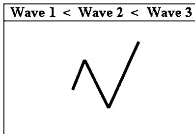
Figure 18-8 Expanding Symmetrical Triangle.
